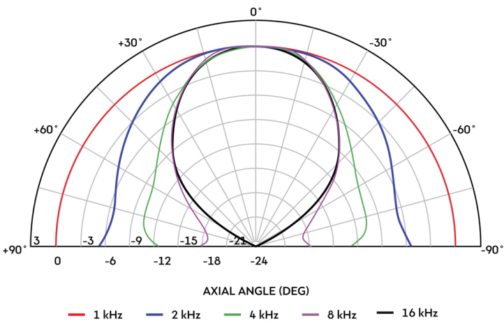
Horizontal Polar
