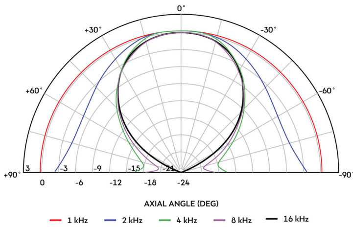
Vertical Polar
