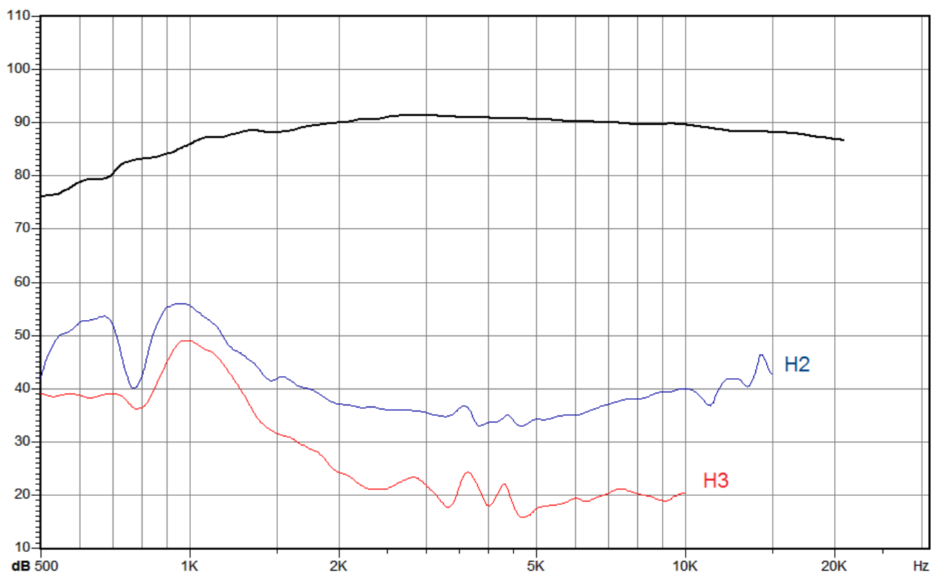
Harmonic distortion at 90 dB
