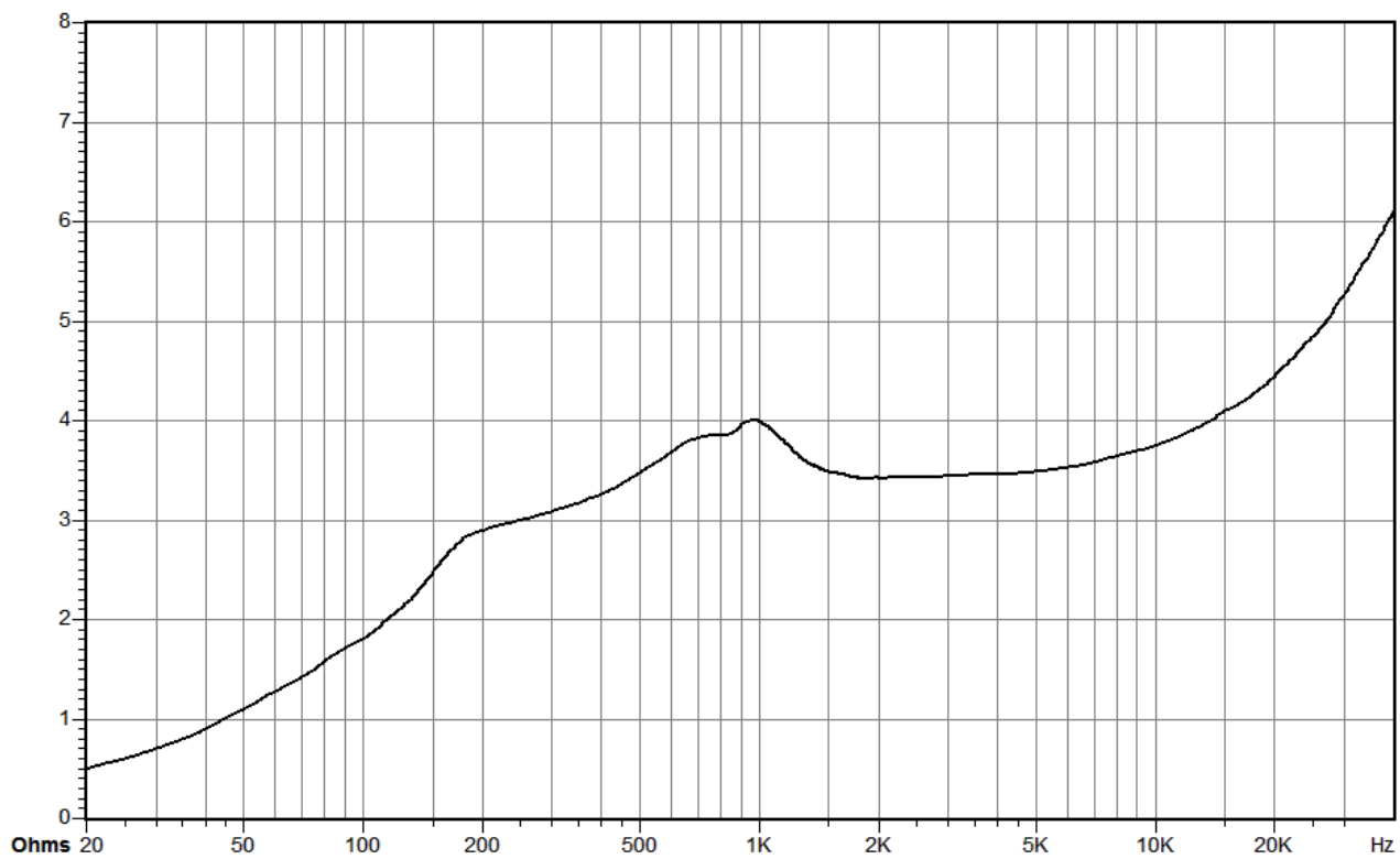
Impedance curve
